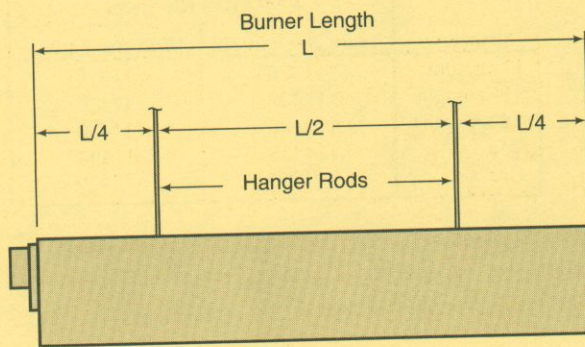
Figure 4c—Burners Over Four Feet Long
