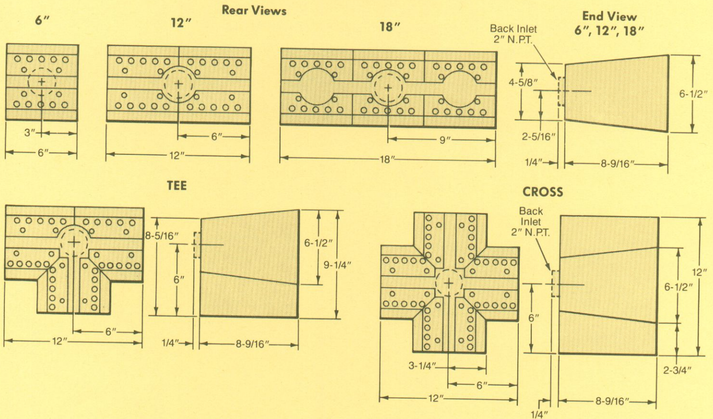
Figure 5—Dimensions
