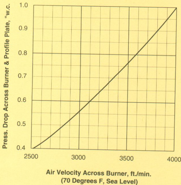
Figure 6— \Delta P VS Air Flow
