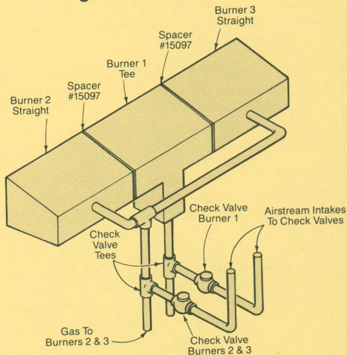
Figure 1—Staged Burners
