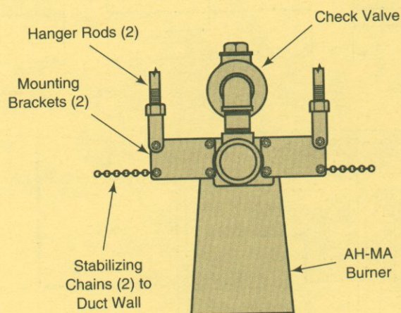
Figure 4b—Burners Up To Four Feet Long, Vertical Firing
