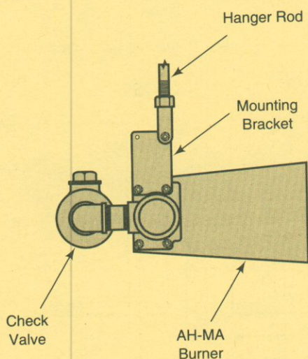
Figure 4a—Burners Up To Four Feet Long, Horizontal Firing
