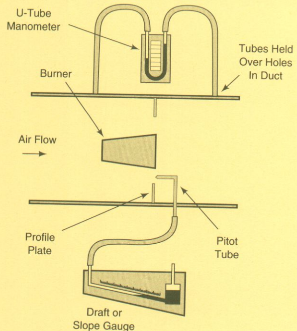
Figure 7—Measuring Duct Pressure
