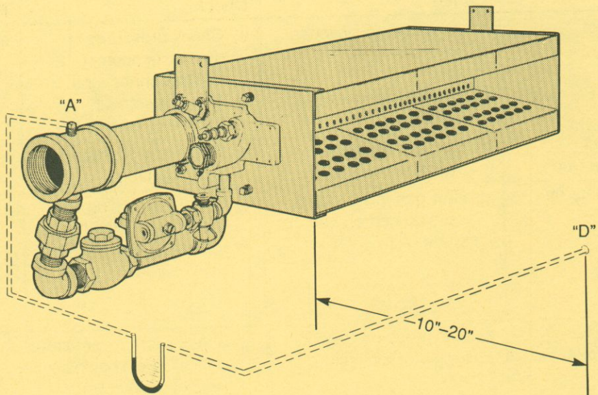
Figure 8—Measuring Gas Differential Pressure
